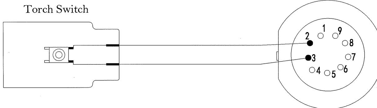
9 Pin Plug
