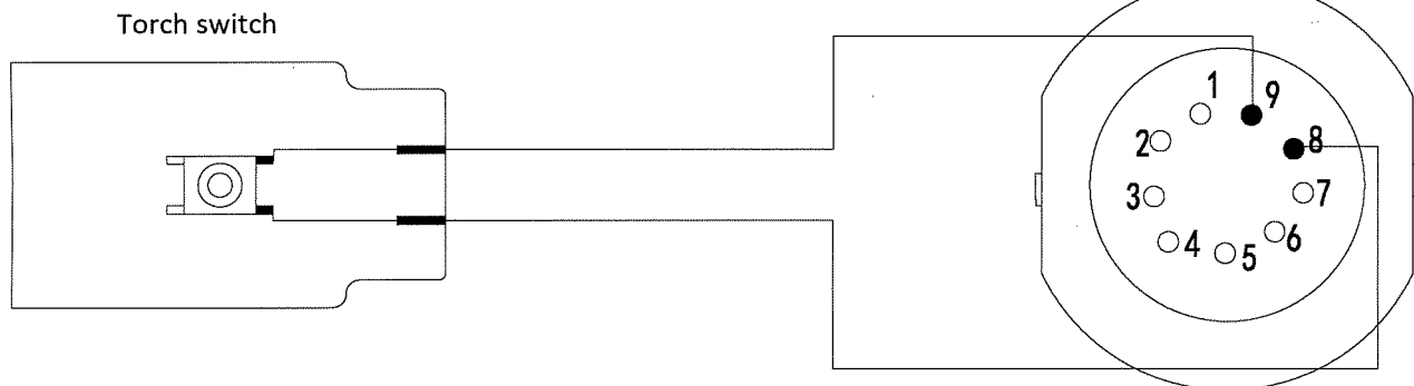
9 Pin plug
