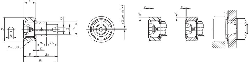
CFE...BR(1) Outside diameter of eccentric collar d_e 16-41mm CFE...B(1) CFE...BUU(1)
